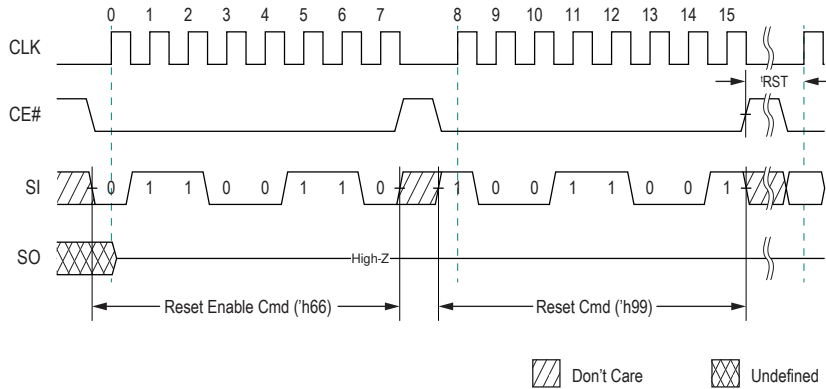
Figure 17: SPI Reset
